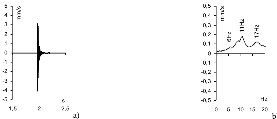
Fig.2.5. The response of the system to pulse induction: a) time course, b) characteristic A-C
