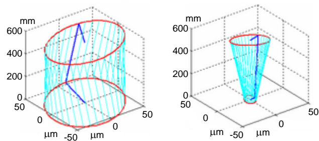
Fig. 3.3. The comparison of the rotor's movement in bearing surfaces a) initial state, b) after the balance, without additional extortion of frame vibrations of frequency of 10.5Hz
